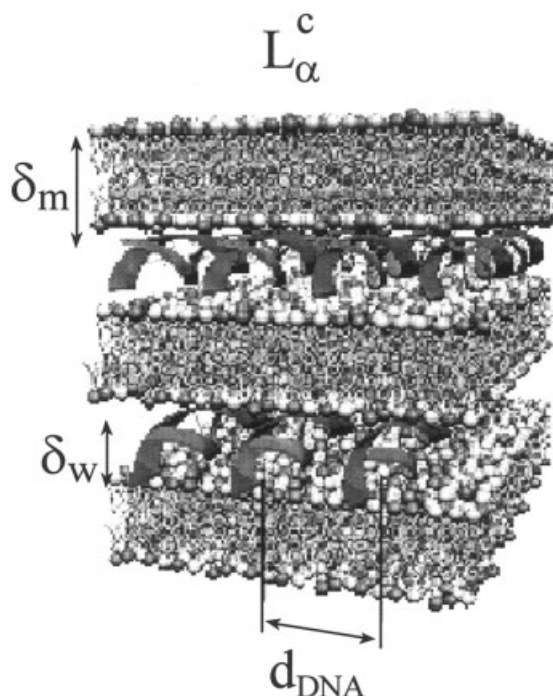
Figure 11. Schematic of the lamellar L_{\alpha}^c phase with alternating lipid bilayers and DNA monolayers of CL–DNA complexes. The interlayer spacing is d = \delta_w + \delta_m .
