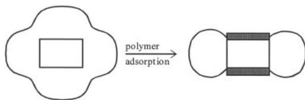
Figure 4. Scheme of vectorial crystal growth. The crystal field (van der Waals and dipole interactions) of a nanocomponent is shielded by the specific polymer adsorption, and objects with tensorial force fields or a heterogeneous distribution of polarity are obtained.
