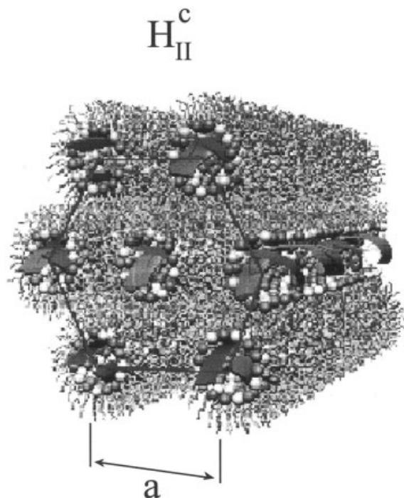
Figure 13. Schematic of the inverted hexagonal H_{II}^c phase (cylinders consisting of DNA coated with a lipid monolayer arranged on a hexagonal lattice) of CL–DNA complexes.
