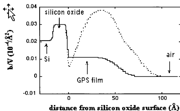
Figure 2. Best-fit scattering length density (SLD) profiles determined by NR (—) before and (---) after swelling with deuterated nitrobenzene vapor of a 5-nm-thick film of crosslinked GPS on an \text{SiO}_x native oxide layer on silicon. (From H. Yim et al., J Phys Chem B , 2002, 106, 2474, adapted by permission.)
