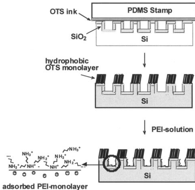
Figure 14. Surface modification procedure used to create wetting contrast in the channels. The treated channels are hydrophobic on the top and hydrophilic inside, and this facilitates the loading and processing of biomaterials in the channels. (From T. Pfohl et al., Langmuir , 2001, 17, 5343, adapted by permission.)
