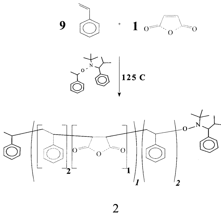
Figure 8. Pseudoblock copolymers prepared in a single step from mixtures of styrene and maleic anhydride are examples of gradient-type macromolecular structures. For instance, a 9:1 mixture of styrene and maleic anhydride gives a tapered block copolymer (2) in which the relative incorporation of maleic anhydride varies from near-alternating at the start of the polymer chain to essentially a pure polystyrene block at the end of the polymer chain.
