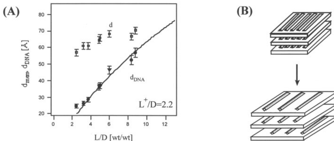
Figure 12. (A) d_{\text{DNA}} and d in the L_{\alpha}^c phase (Fig. 2) plotted as functions of the lipid/DNA ( L/D ; w/w) ratio at an isoelectric point of 2.2 for the DOTAP/DNA complex. d_{\text{DNA}} expands from 24.5 to 57.1 Å. The solid line through the data is the prediction of a packing calculation in which the DNA chains form a space-filling 1D lattice. (B) Schematic of DNA–membrane multilayers showing an increase in the distance between DNA chains as the membrane charge density is reduced (as \Phi_{\text{DOPC}} increases) at the isoelectric point. (From J. O. Raedler et al., Science , 1997, 275, 810; J. O. Raedler et al., Langmuir , 1998, 14, 4272; and I. Koltover et al., Science , 1998, 281, 78, adapted by permission.)
