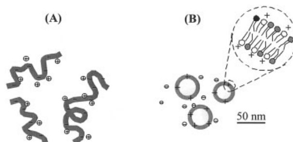
Figure 10. (A) Linear DNA with cationic counterions condensed on the backbone because of Manning condensation and (B) CLs (spherical membranes or vesicles) containing a bilayer of a mixture of cationic and neutral lipids.
