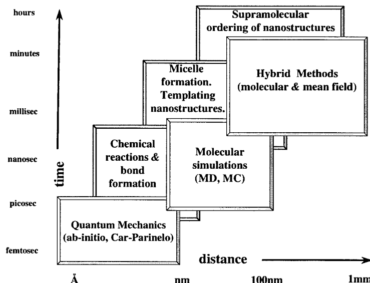
Figure 6. Schematic illustration of the vast span of length scales (angstroms to macroscopic) and timescales (femtoseconds to macroscopic), which present a challenge to realistic simulations. The simulation methods presently suited to the indicated span of length scales and timescales are shown.
