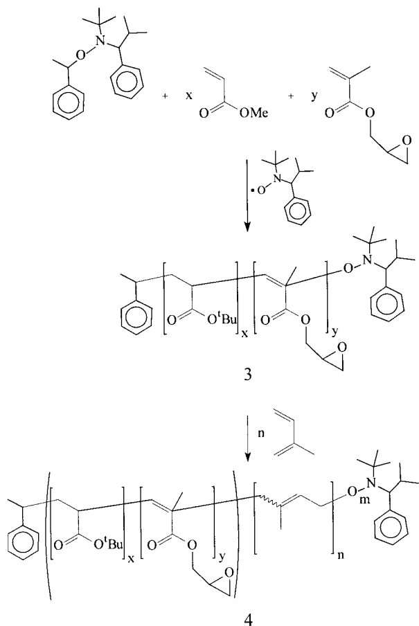
Figure 9. Random block copolymers bear a greater resemblance to traditional block copolymers, in that there are two discrete blocks, with at least one being composed of a random copolymer segment. An excellent example of the synthesis and application of these materials is the preparation of the functionalized block copolymer 4 . An initial random copolymer of methyl acrylate and glycidyl methacrylate ( 3 ) can be prepared by nitroxide-mediated living free-radical polymerization and used to initiate the polymerization of isoprene, which leads to 4 .
